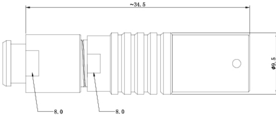
CONNECTOR SOLDER CUP VIEW
