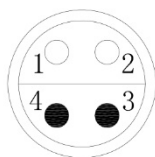
CONNECTOR SOLDER CUP VIEW
