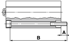
Axial mounting
