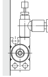
Mounting condition 1
