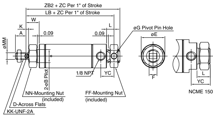
Double end mount / Spring return NCME_-_S
