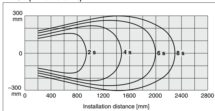
IZF31 (Air flow level: 10)
