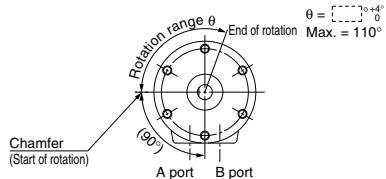
Start of rotation is the position of the chamfer (key) when B port is pressurized. The above figure shows the CRB2 series. (Viewed from the long shaft side)
