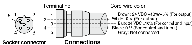
Socket connector pin arrangement B-coded (Reverse key)
