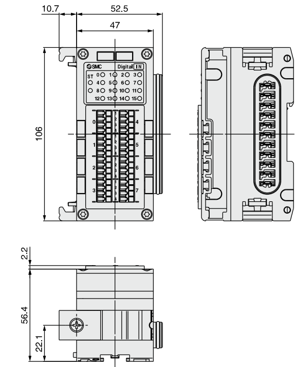
EX600-DX□F EX600-DY□F EX600-DM□F
