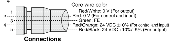
Socket pin arrangement
