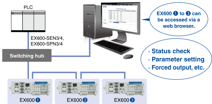
Connection example
