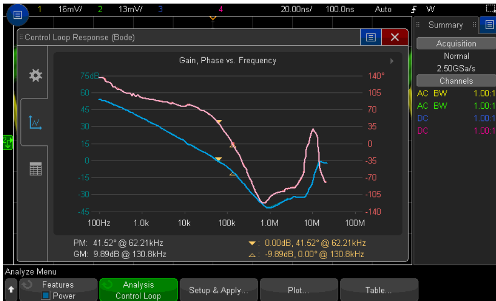
Figure 3. Control loop response test using the DSOX3054PWR Power Better Bundle.
