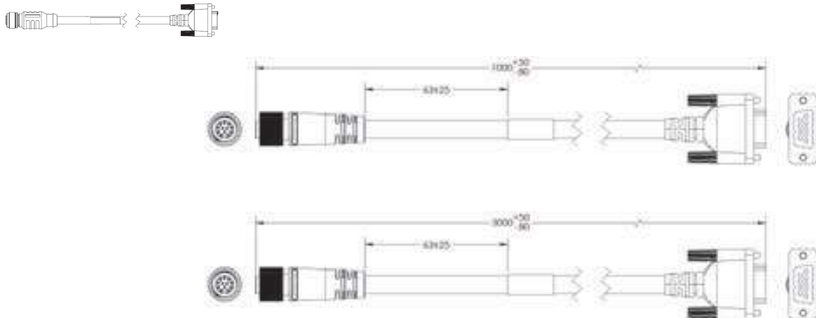
M12 to RS-232 Breakout – 1 Meter or 3 Meters V430-WR-1M V430-WR-3M
