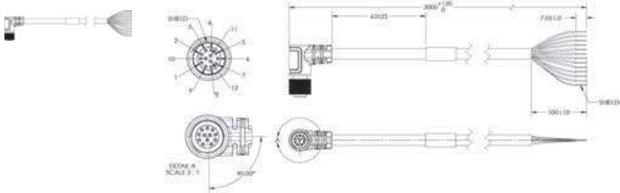
M12 to Flying Leads Cable Right Angle Down Power, IO, RS232, USB – 3 Meters V430-W8LD-3M
