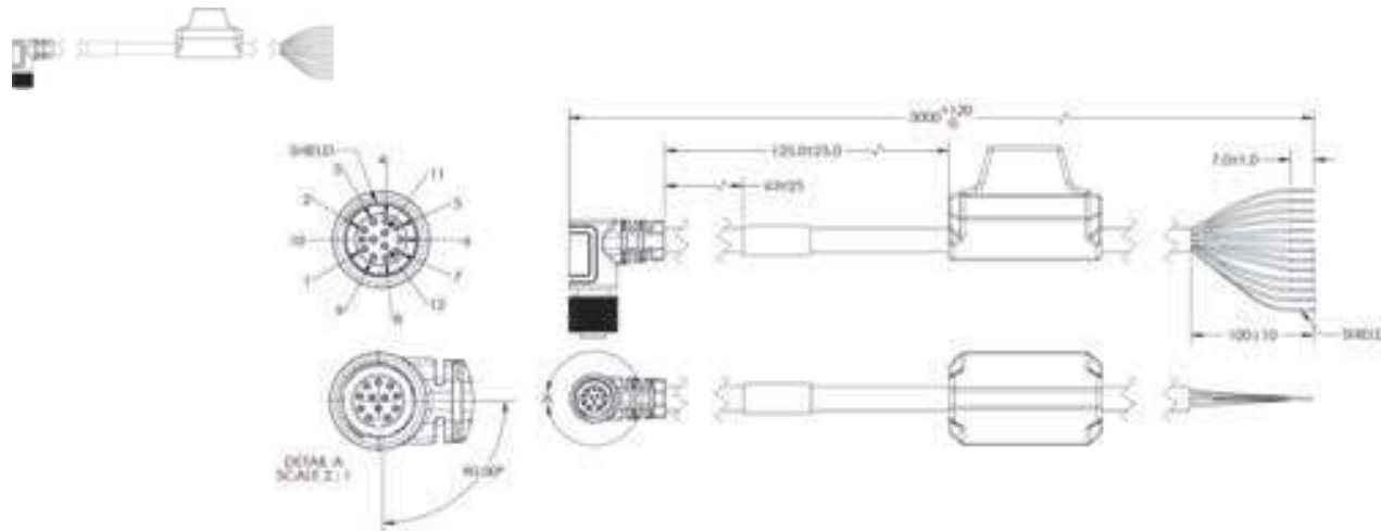
M12 to Flying Leads Cable Right Angle Down, with Power Filter – 3 Meters V430-W8LDF-3M
