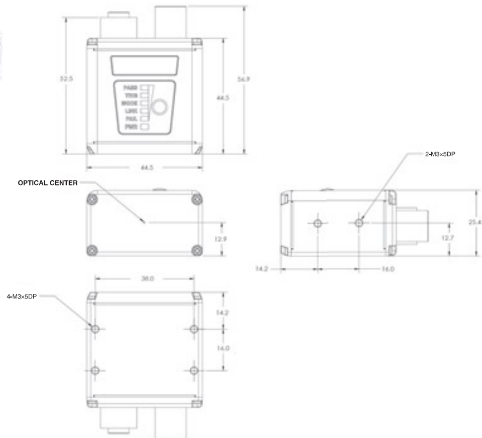
V430-F with Alternate Optics and Illumination
