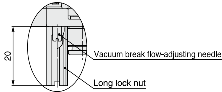
For individual port exhaust (Body type: F)
