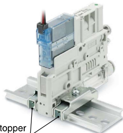
Stopper
