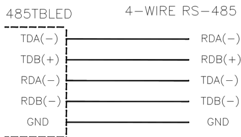
Figure 2. 4-Wire RS-485
