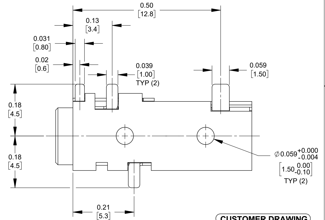
Ø3.5MM MATING PLUG
