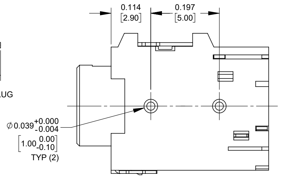
CUSTOMER DRAWING
