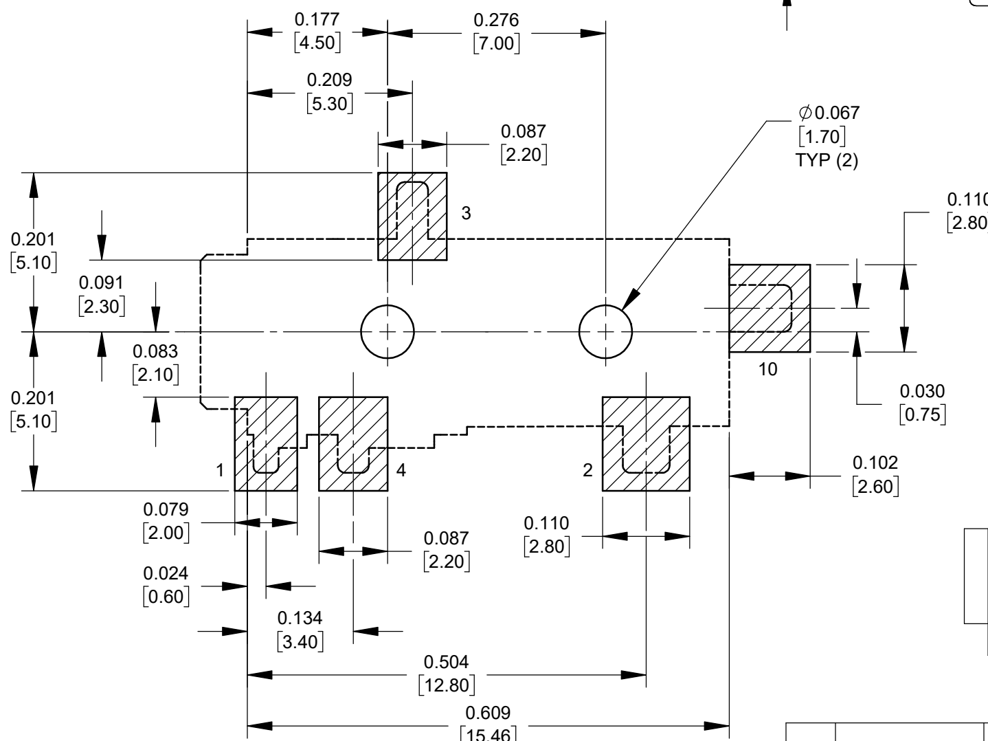
PCB LAYOUT COMPONENT SIDE
