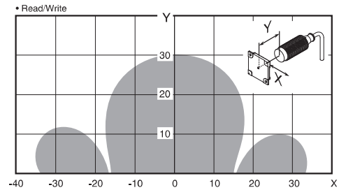
V680-HS65 (mounted on metallic material) & V680S-D8KF67M (mounted on metallic surface: steel)
