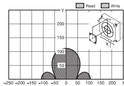
V680-HS63 (mounted on non-metallic material) & V680S-D2KF67M (mounted on metallic surface: steel)
