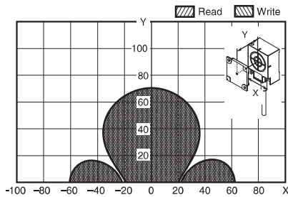
V680-H01-V2 (mounted on non-metallic material) & V680S-D2KF67 (mounted on non-metallic material)
