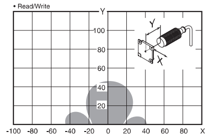
V680-HS65 (mounted on metallic material) & V680S-D8KF67
