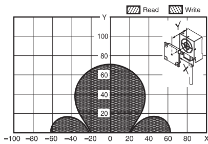
V680-HS52 (embedded in non-metallic material) & V680S-D2KF67M (mounted on metallic surface: steel)
