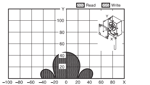
V680-HS63 (with Metal on Back Surface) & V680S-DKF68 (Tag direction: Horizontal)
