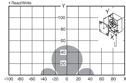
V680-HS63 (mounted on non-metallic material) & V680S-D8KF67
