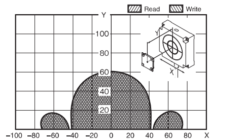
V680-HS63 (with Metal on Back Surface) & V680S-DKF68 (Tag direction: Vertical)
