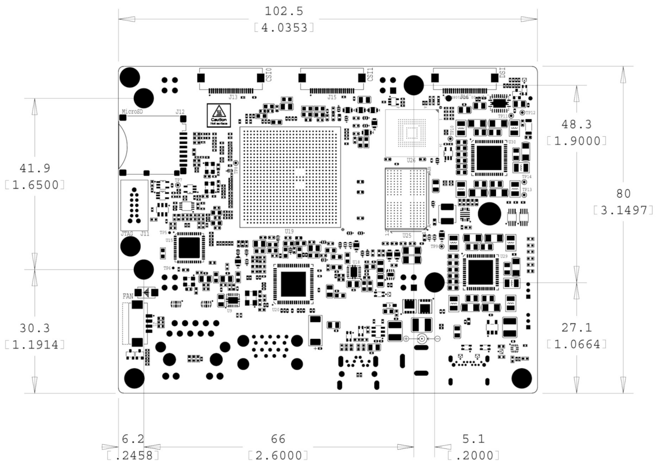
Figure 20. Board Dimensions
