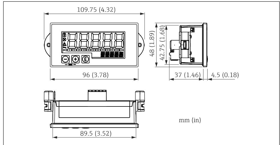
29 Dimensions of the panel housing
