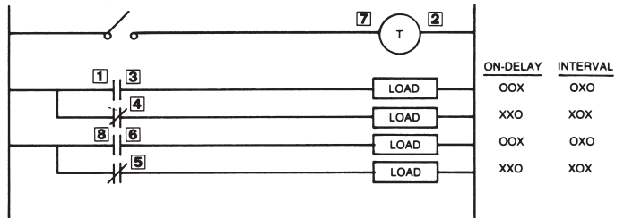
*For Interval Operation with a Momentary Start Switch, Jumper 7 & 3
