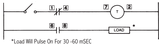
*Load Will Pulse On For 30 -60 mSEC
