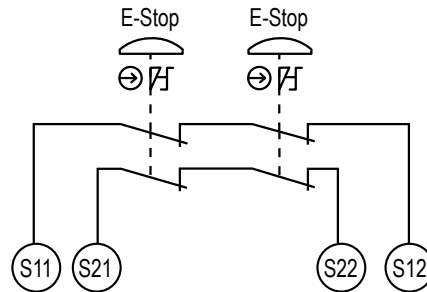
Figure 2. Series connection of multiple E-stop switches
