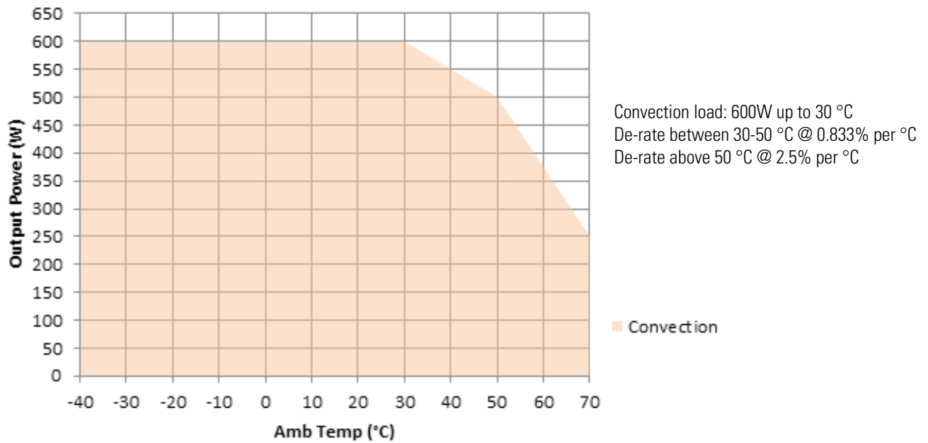
Derating Curve 24 V & above
