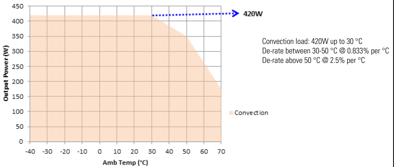
Derating Curve 24 V & above for slotted cover
