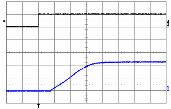
Fig. 8: Turn-on transient at full rated load current (resistive) plus 2,200 µF at Vin = 56 V, triggered via ON/OFF pin. Top trace: ON/OFF signal (5 V/div.). Bottom trace: output voltage (5 V/div.). Time scale: 2 ms/div.
