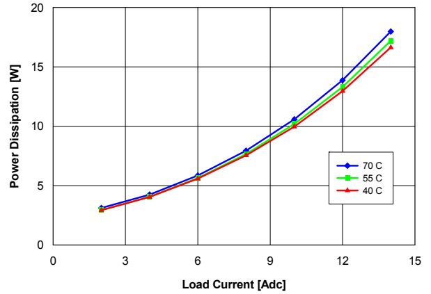
Fig. 6: Power dissipation vs. load current and ambient temperature for converter mounted horizontally with Vin = 48 V and air flowing from pin 3 to pin 1 at a rate of 200 LFM (1.0 m/s).
