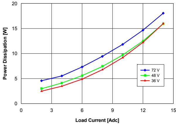
Fig. 5: Power dissipation vs. load current and input voltage for converter mounted horizontally with air flowing from pin 3 to pin 1 at a rate of 300 LFM (1.5 m/s) and Ta = 25 °C.
