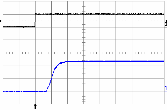
Fig. 7: Turn-on transient at full rated load current (resistive) with no output capacitor at Vin = 56 V, triggered via ON/OFF pin. Top trace: ON/OFF signal (5 V/div.). Bottom trace: output voltage (2 V/div.). Time scale: 2 ms/div.
