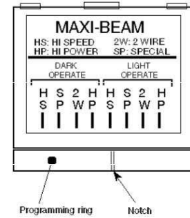
Figure 1. Sensor Head and Programming Ring
