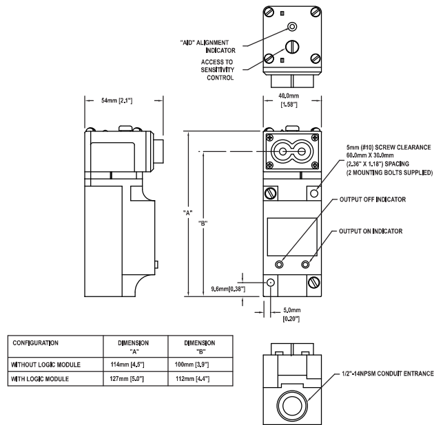
Figure 4. Dimensions for the fiber models
