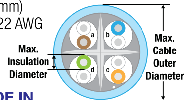
CABLE DIAGRAM
