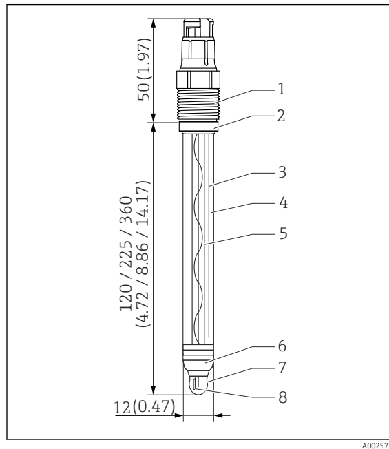
8 CPS11D with Memosens plug-in head, temperature sensor
