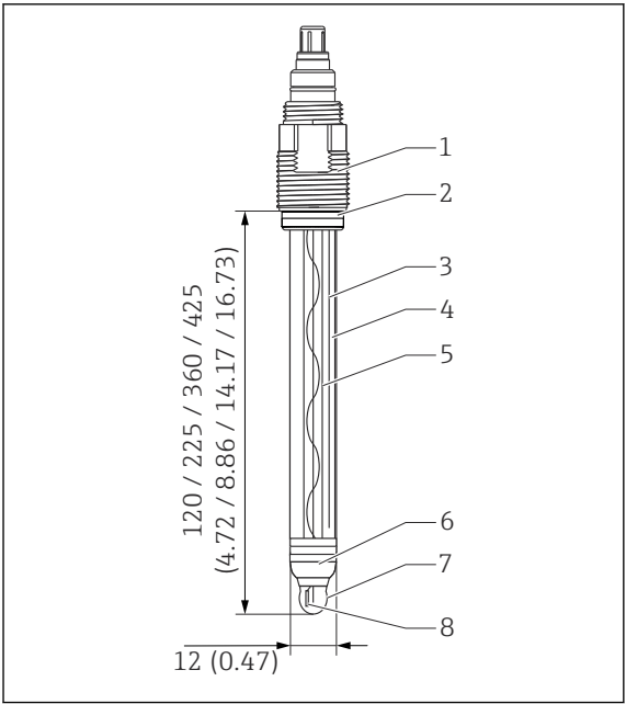
11 CPS11 with TOP68 plug-in head, temperature sensor
