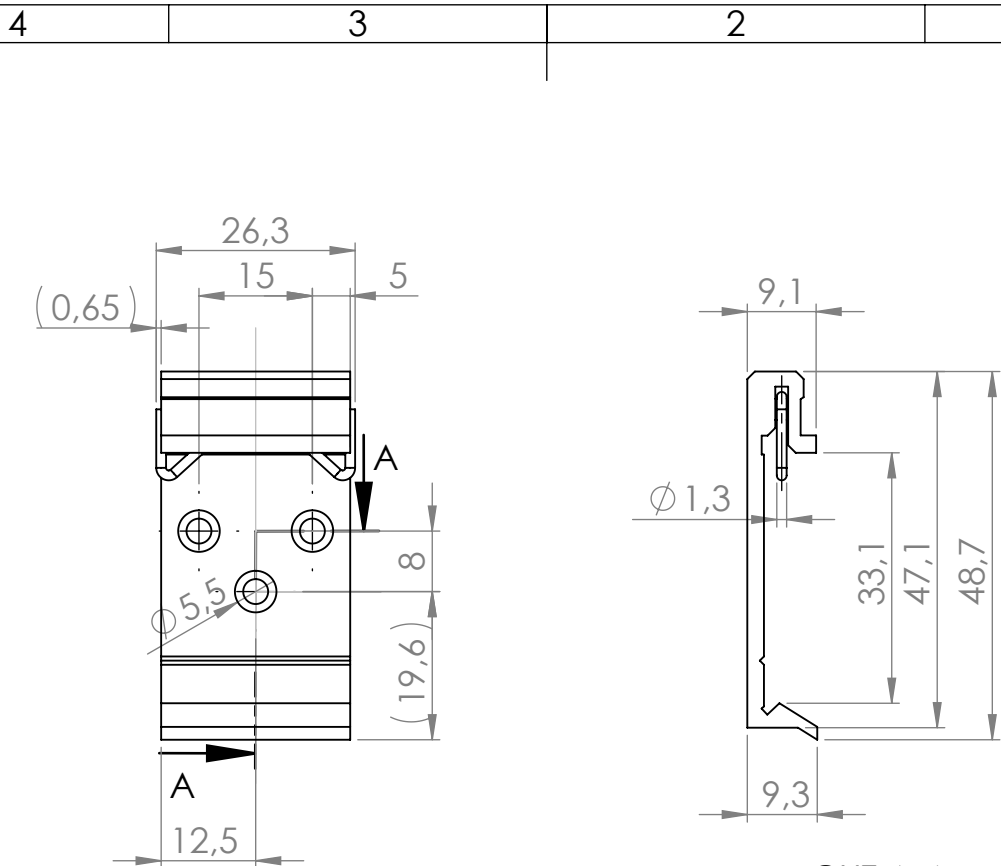
CUT A-A SCALE 2 : 1
