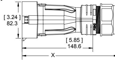
APPROXIMATE OVERALL LENGTH W/ GLAND X
