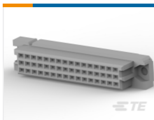
TE Part # 5535070-5 ASSY,RECEPTACLE,EUROCARD,TYPE
