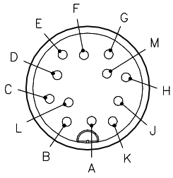
M16 connector
