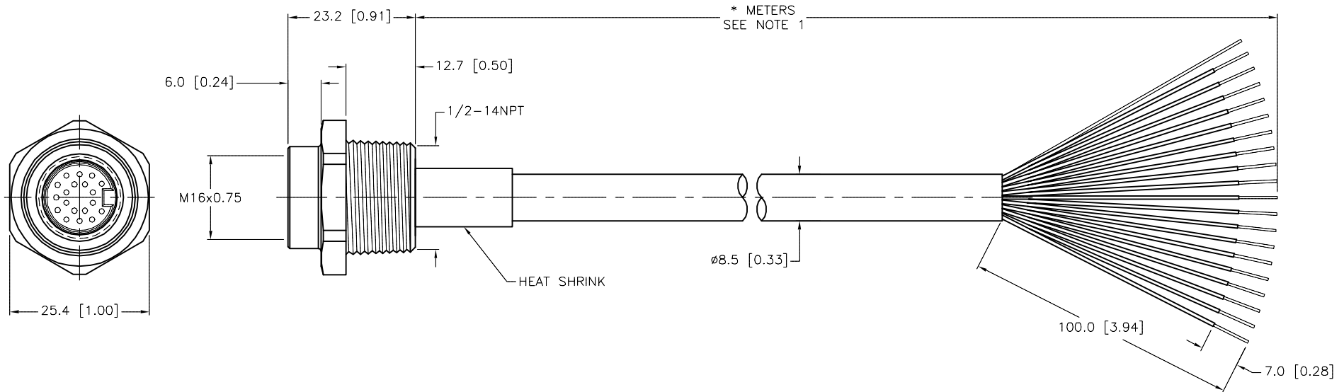
M16 connector
