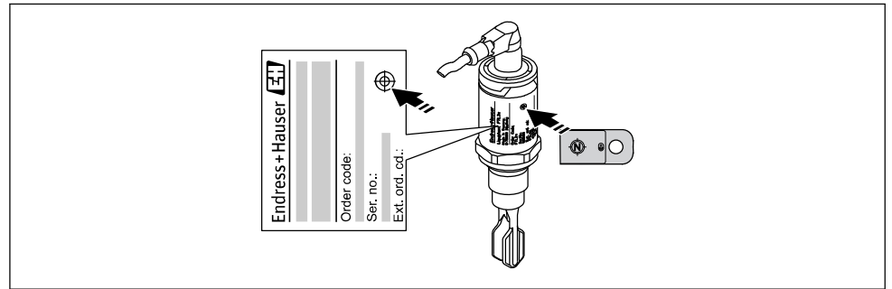
23 Position for test magnet on housing
